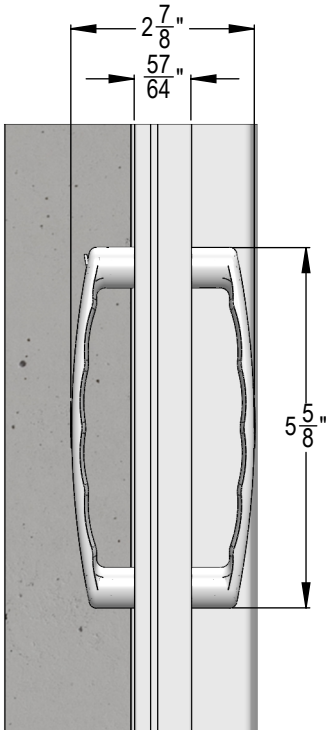
SIDE VIEW OF HANDLES & PULL BAR
