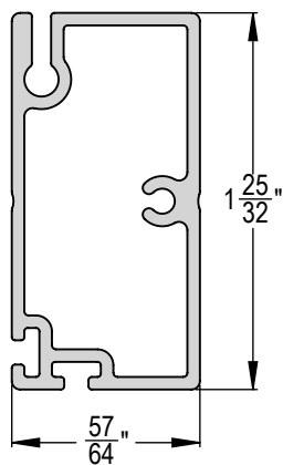
SIDE VIEW OF PULL BAR
