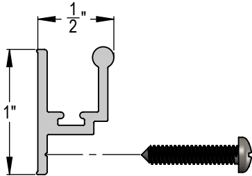
SIDE VIEW OF RAIL
