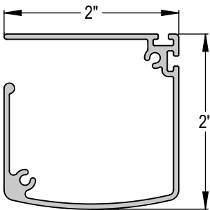
SIDE VIEW OF HOUSING
